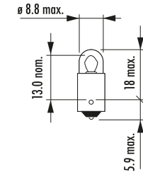
W5W Halogen, 70761
