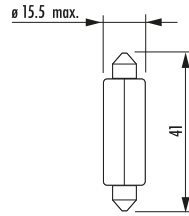
C21W, 17512, 17522
