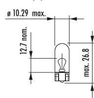
W2, 2W, W3W, W(Y)5W, 17069
