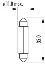
C5W, 17316
