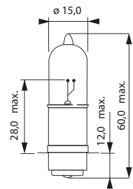
M5 (P15d-25-3)
