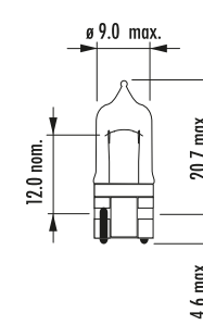
W5W Halogen, 70761
