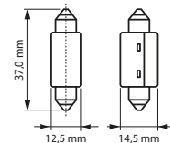
Festoon 10,5x38 LED
