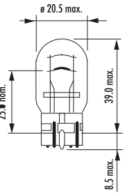
W21/5W
