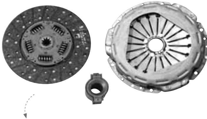
Kit embrayage diam 280 mm, 10 dents Ref. 171052021 Ref OE 2994020
