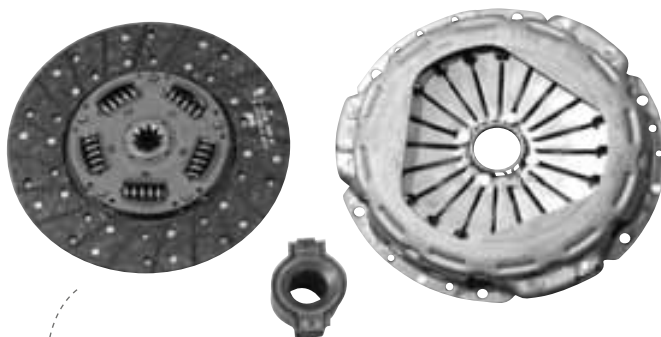
Kit embrayage diam 280 mm, 10 dents Ref. 171052021 Ref OE 2994020
